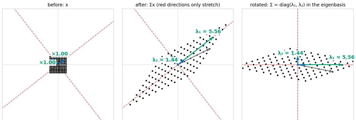
Figure 1.1: The map \mathbf{x} \mapsto \Sigma \mathbf{x} acting on a grid of points (left: before; middle: after). Points on the two dashed red eigen-directions only slide along them; each eigenvector (blue) is stretched by its eigenvalue (green): \lambda_1 \approx 5.56 and \lambda_2 \approx 1.44 . The grey vector, not an eigenvector, changes direction. Right: rotating until the eigenvectors are the axes, \Sigma is nothing but a stretch along each axis. (The HTML version of these notes animates this.)
