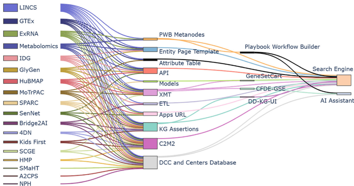
Figure 1. (A) The CFDE Workbench receives metadata, processed data, and code assets from the CF program participating DCCs. These assets are uploaded via a data submission system and assessed for FAIRness with FAIRshake. Approved uploads are displayed in a Data Matrix and served via a search engine. The metadata, processed data, and code assets enable the development of a layer of tools that include the PWB [44], GeneSetCart [47], DD-KG-UI [46], and CFDE-GSE. (B) Sankey diagram demonstrating how processed data and metadata items from the various DCCs flows into the CFDE Data Portal and then feed the CFDE Workbench tools, the search engine and the AI Assistant.
