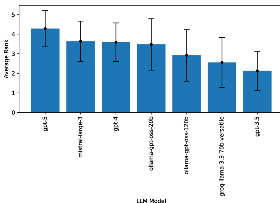
Figure 8. All example questions were submitted to each LLM and then organized randomly into an online survey where responses were scored for answer between 0–5 (5-best). Eight human reviewers evaluated the answers independently.
