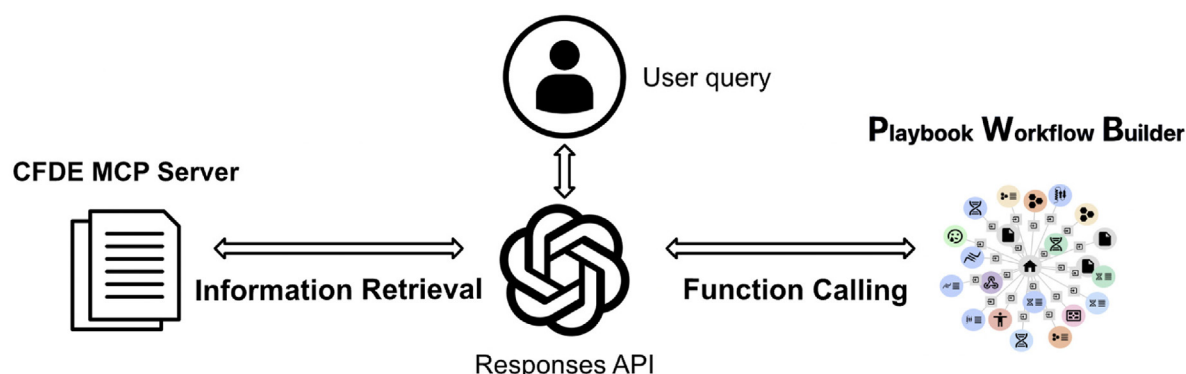
Figure 7. The CFDE Workbench AI Assistant uses OpenAI's Responses API to send user queries to GPT-4. The LLM then queries the CFDE MCP server and selects an appropriate tool based on the query. These tools provide information about the CFDE, the different centers, and the different Common Fund Programs involved in the consortium. Additionally, there are tools that define several workflows from the Playbook Workflow Builder that utilizes and integrates data from the different CF Programs and are available for users to interact with via the chat interface.
