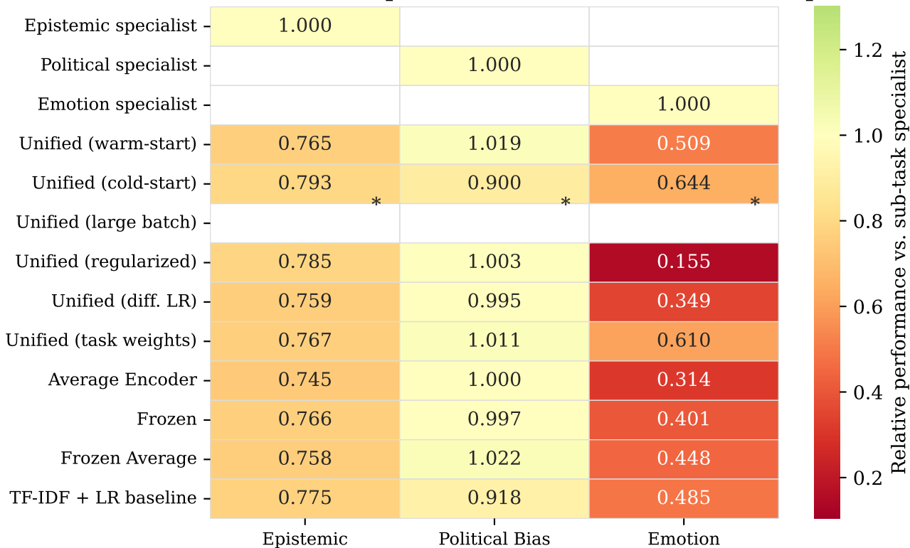
Performance heatmap (models × tasks, latest checkpoint)
