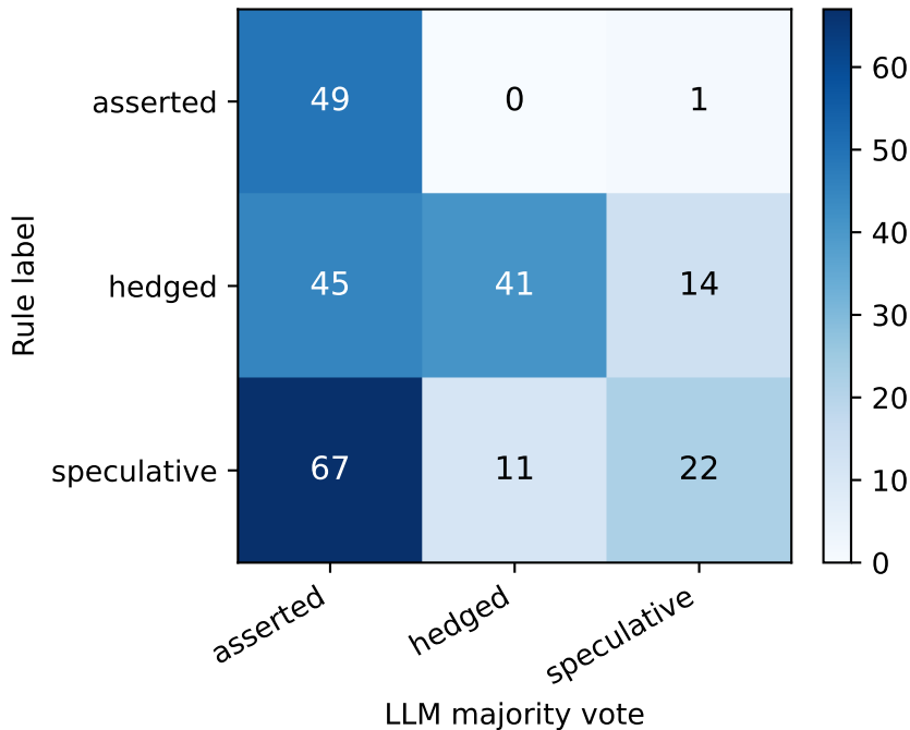
Rule vs. LLM agreement ( \kappa = 0.243 , fair)
