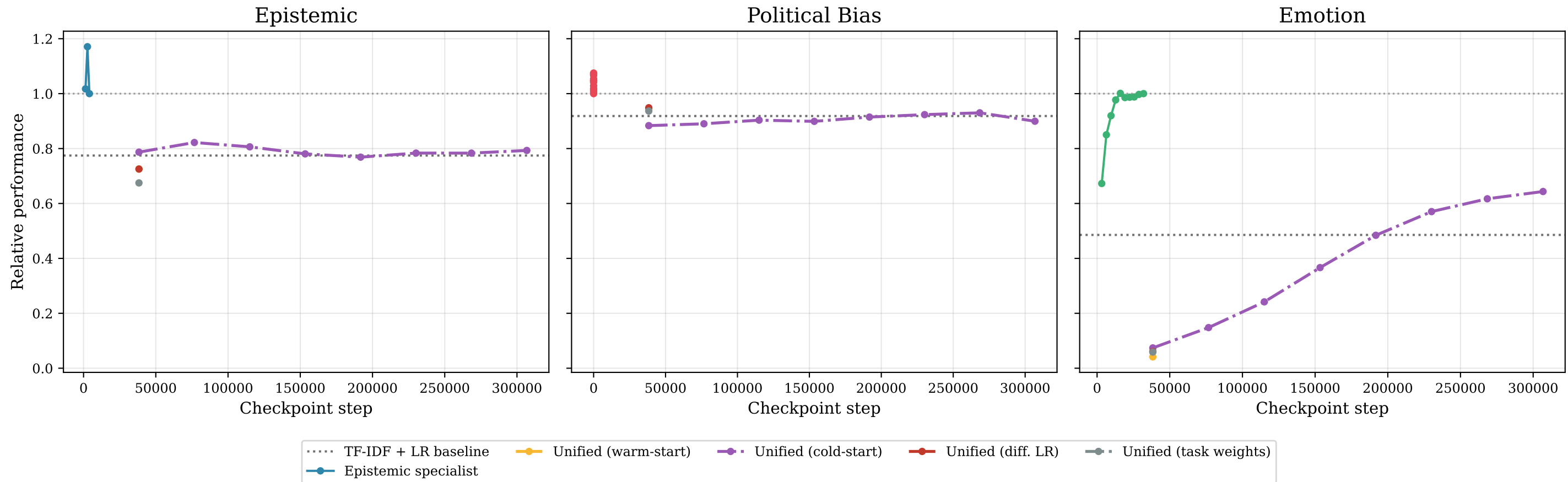
Training curves by task
