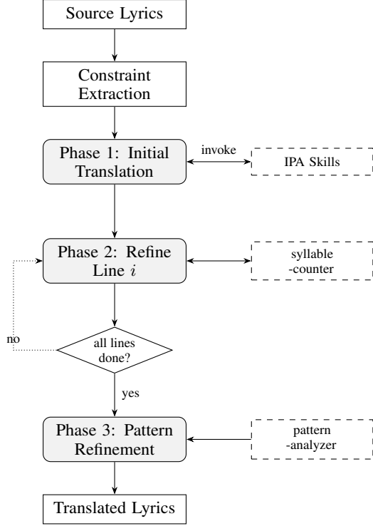
Figure 1: Skill framework overview. Phase 1 translates all lines using an internal tool-use loop that invokes the IPA skills. Phase 2 refines each line sequentially (up to 10 attempts per line); the dotted arrow shows the orchestration loop that iterates through lines. Phase 3 is a single pass that uses the syllable-pattern-analyzer skill output to guide pattern refinement without a retry loop.
