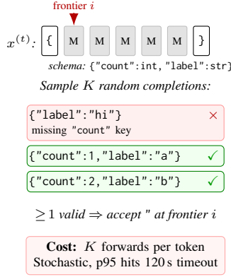
Figure 1: One denoising step under schema {"count":int, "label":str}. LAVE (Zhang et al., 2026) (left) samples K random completions at each frontier token, accepting it only when \geq 1 suffix is valid; stochastic and K\times more expensive per token, hitting the 120 s per-instance timeout on hard schemas. Dgrammar (right) runs compute_mask on the incremental FSM state and unmask an entire block under that mask in one forward pass, overlapped with the next mask computation; the result is deterministic. The figure is illustrative; LAVE’s actual cost depends on its retry schedule and verifier policy (see §2).
