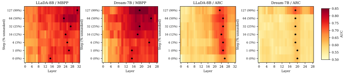
Figure 4: AUC heatmaps for MBPP and ARC-Challenge. Both show gradual emergence similar to GSM8K. ARC has the weakest overall signal ( \text{AUC} \leq 0.75 ).
