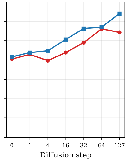
MBPP
