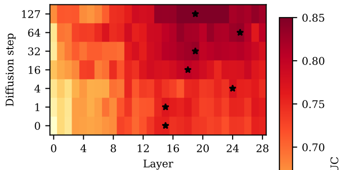
Dream-7B / MBPP
