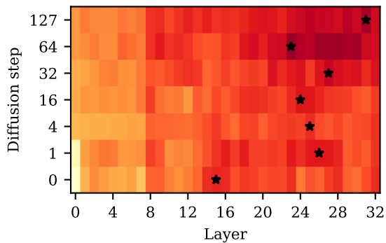
LLaDA-8B / MBPP
