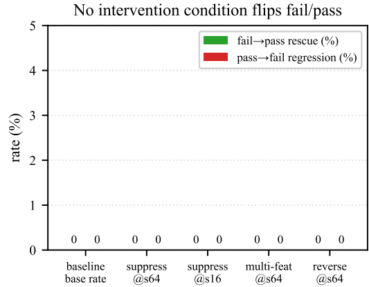
Figure 3: Five steering conditions on LLaDA-8B / MBPP cluster-1 fails ( n=8 ) and a pass regression control ( n=3 ). Conditions: baseline (no intervention); suppress f_{15601} at step 64 (SAE training window); suppress f_{15601} at step 16 (pre-peak); suppress the top-5 fail features at step 64; reverse intervention ( \alpha = -5 ) adding f_{15601} at step 64. No condition converts any fail→pass or pass→fail.
