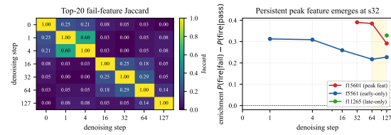
Figure 4: Left: pairwise Jaccard of top-20 fail features between denoising steps. Right: enrichment trajectory of f15601 (persistent peak), f5561 (OOD early only), and f11265 (final only).
