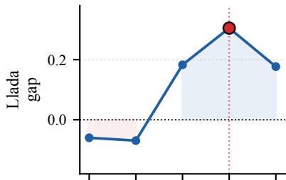
MBPP (code)
