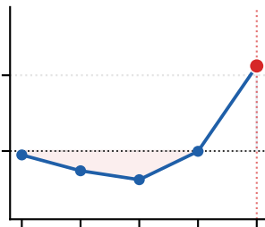
GSM8K (math)
