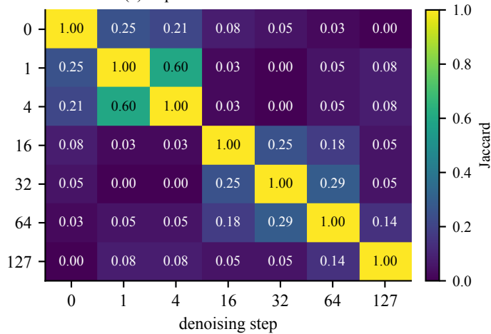
(a) Top-20 fail-feature Jaccard
