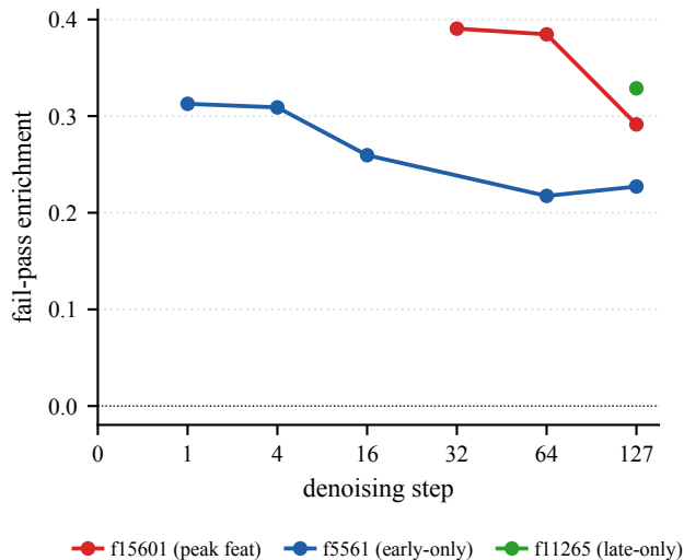
(b) Persistent peak feature emerges at s32
