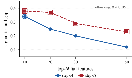
Figure 7: Signal-to-null gap as the top- N fail-feature cutoff is varied at LLaDA-MBPP plateau steps 64 and 68. Hollow rings mark p < 0.05 . Step 68 is robust across N ; step 64 only reaches significance at N=10 .
