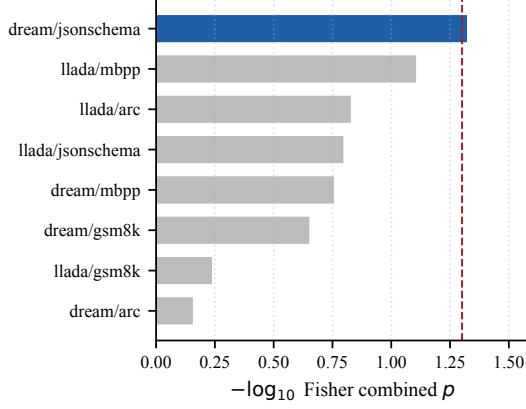
Figure 8: Fisher combined p across the sparse 5-step grid for each of the 8 (DLM, task) cells. Dream-JSON reaches aggregated significance ( p = 0.047 ); LLaDA-MBPP is next strongest. The dashed line marks p = 0.05 .
