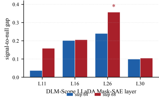
Figure 7: LLaDA-MBPP signal-to-null gap across SAE layers at plateau steps 64 and 68. L26 is the unique layer where the gap reaches permutation p < 0.05 (step 68, gap +0.357, p = 0.006 ). Top-1 fail-enriched feature varies by layer; f15601 appears only at L26.
