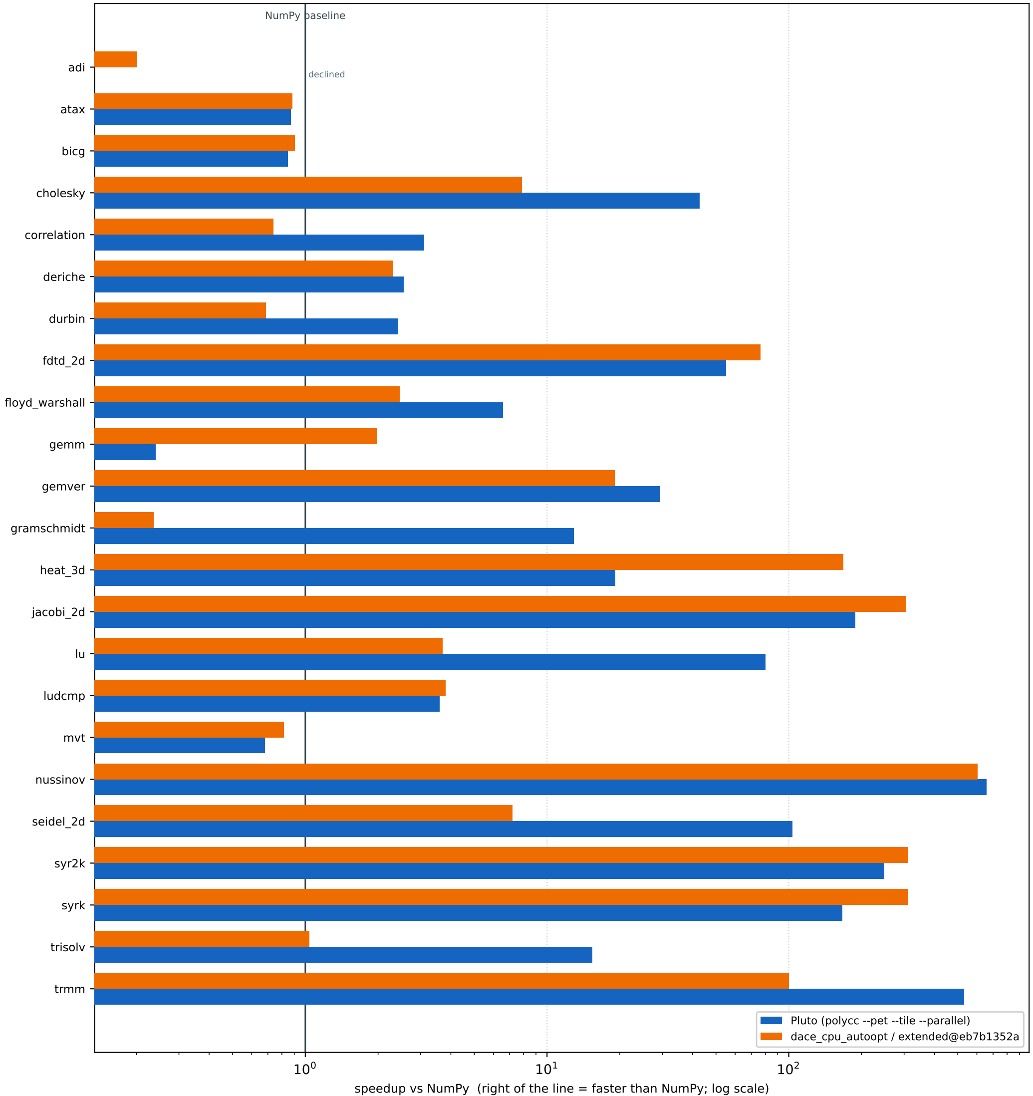
NPBench PolyBench-derived kernels preset paper, REPEAT=50 - VERIFICATION RUN, not a performance measurement DaCe column = dace_cpu_autoopt / extended@eb7b1352a
