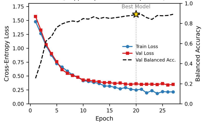
Fold 0 (stopped epoch 27, best epoch 20)
