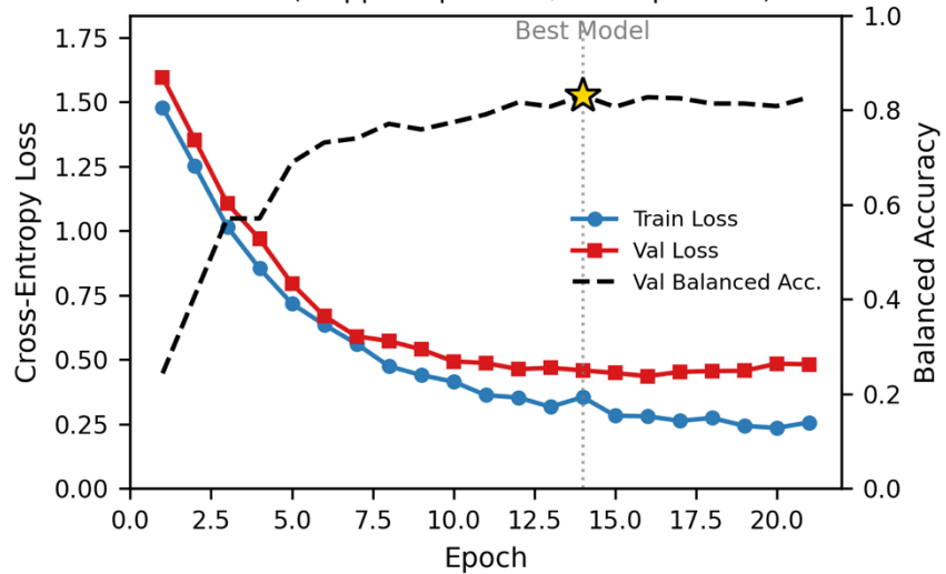
Fold 1 (stopped epoch 21, best epoch 14)
