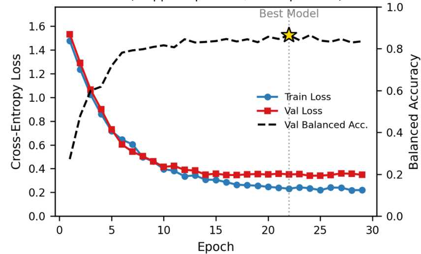
Fold 2 (stopped epoch 29, best epoch 22)
