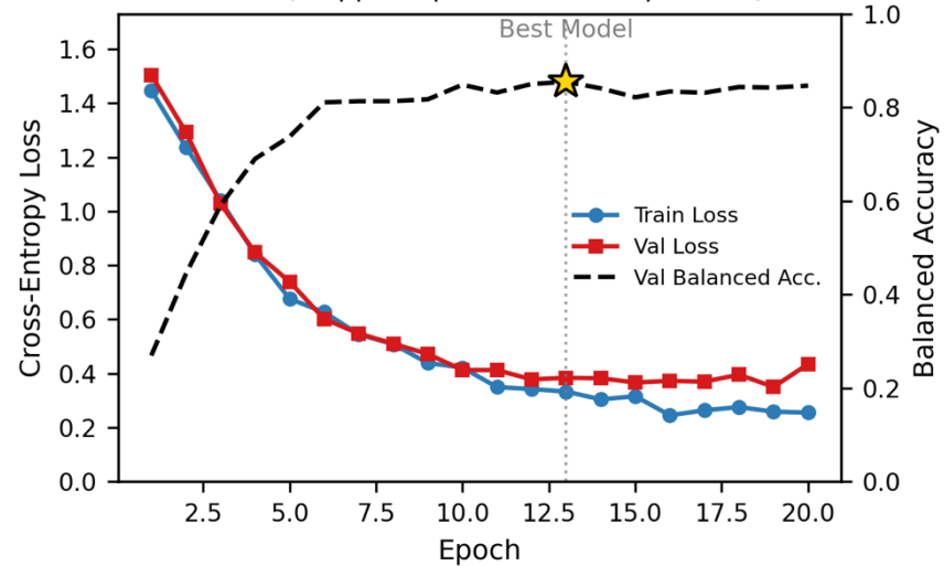
Fold 3 (stopped epoch 20, best epoch 13)
