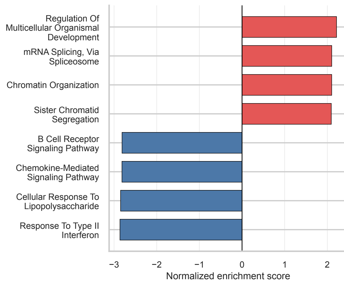
GO Biological Process
