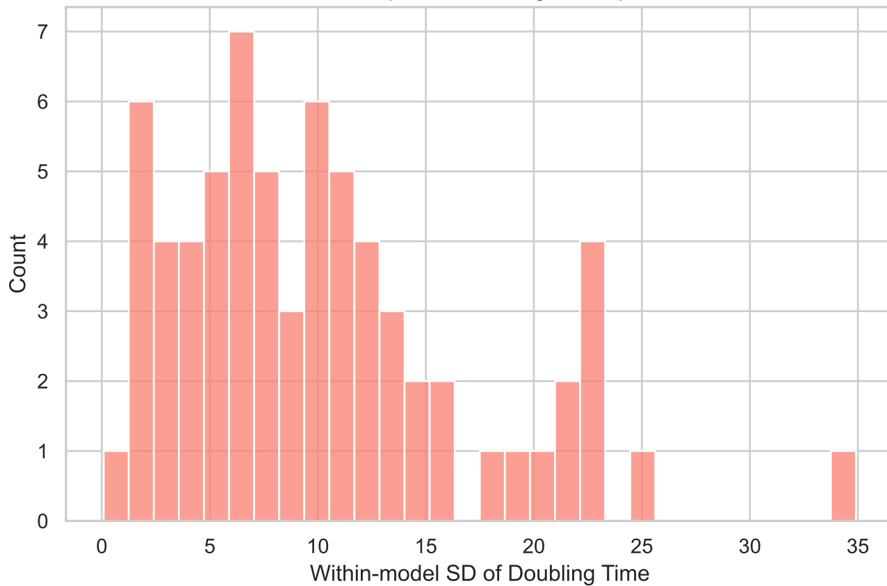
Variation of Replicate Doubling Times per Model
