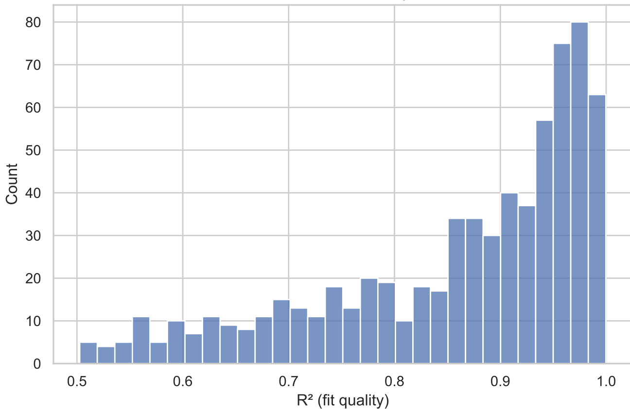
Distribution of R^2 Values for Exponential Fits
