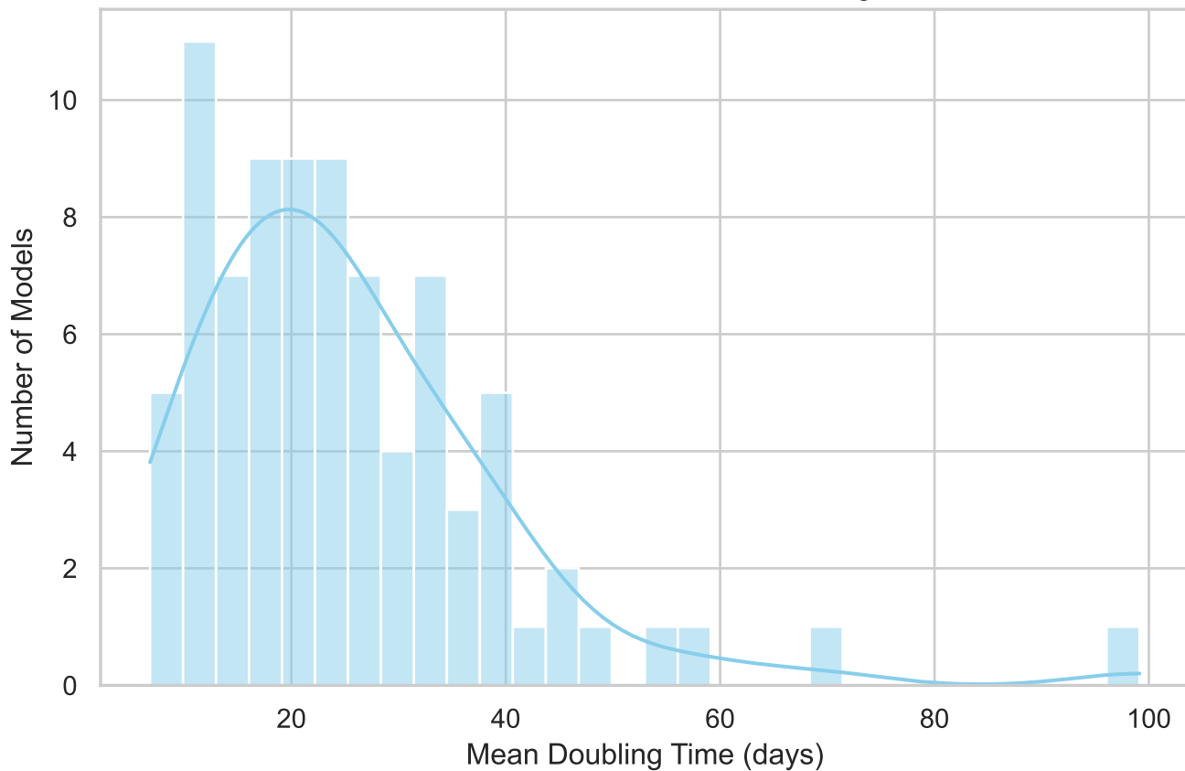
Distribution of Model-level Mean Doubling Times
