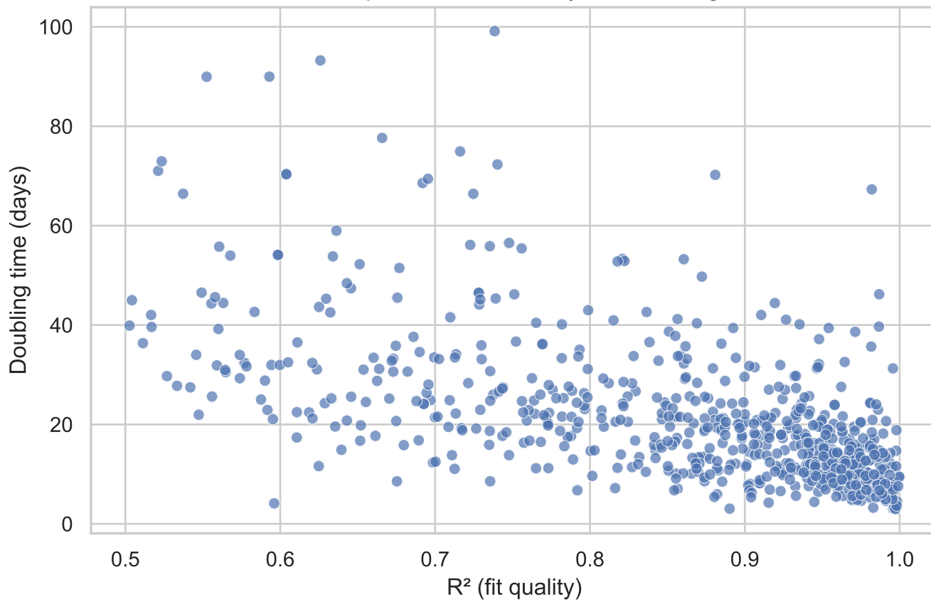
Relationship between Fit Quality and Doubling Time
