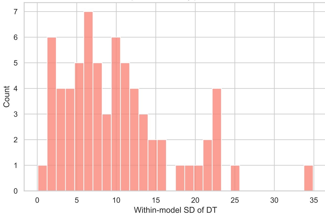
Replicate Variability per Model
