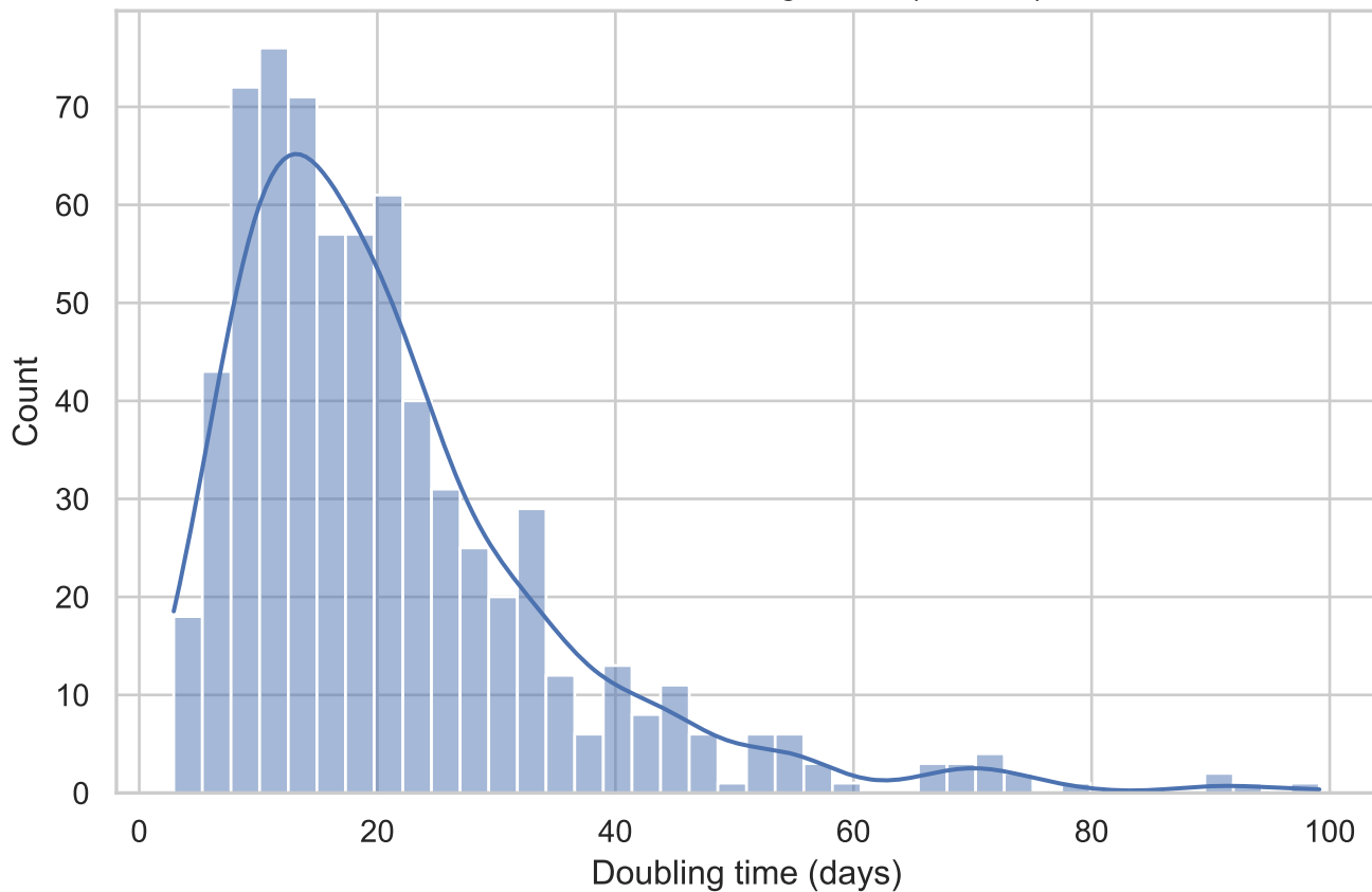
Distribution of Doubling Times (all mice)
