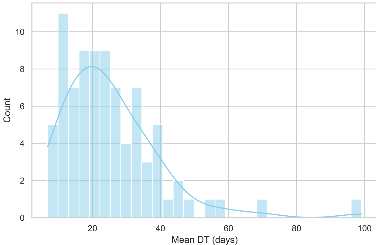
Model-level Mean Doubling Times
