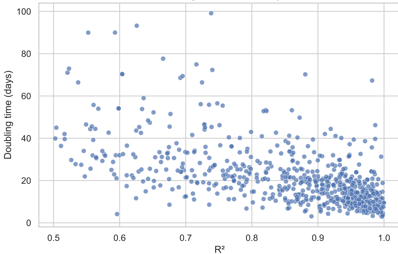
Doubling Time vs. Fit Quality
