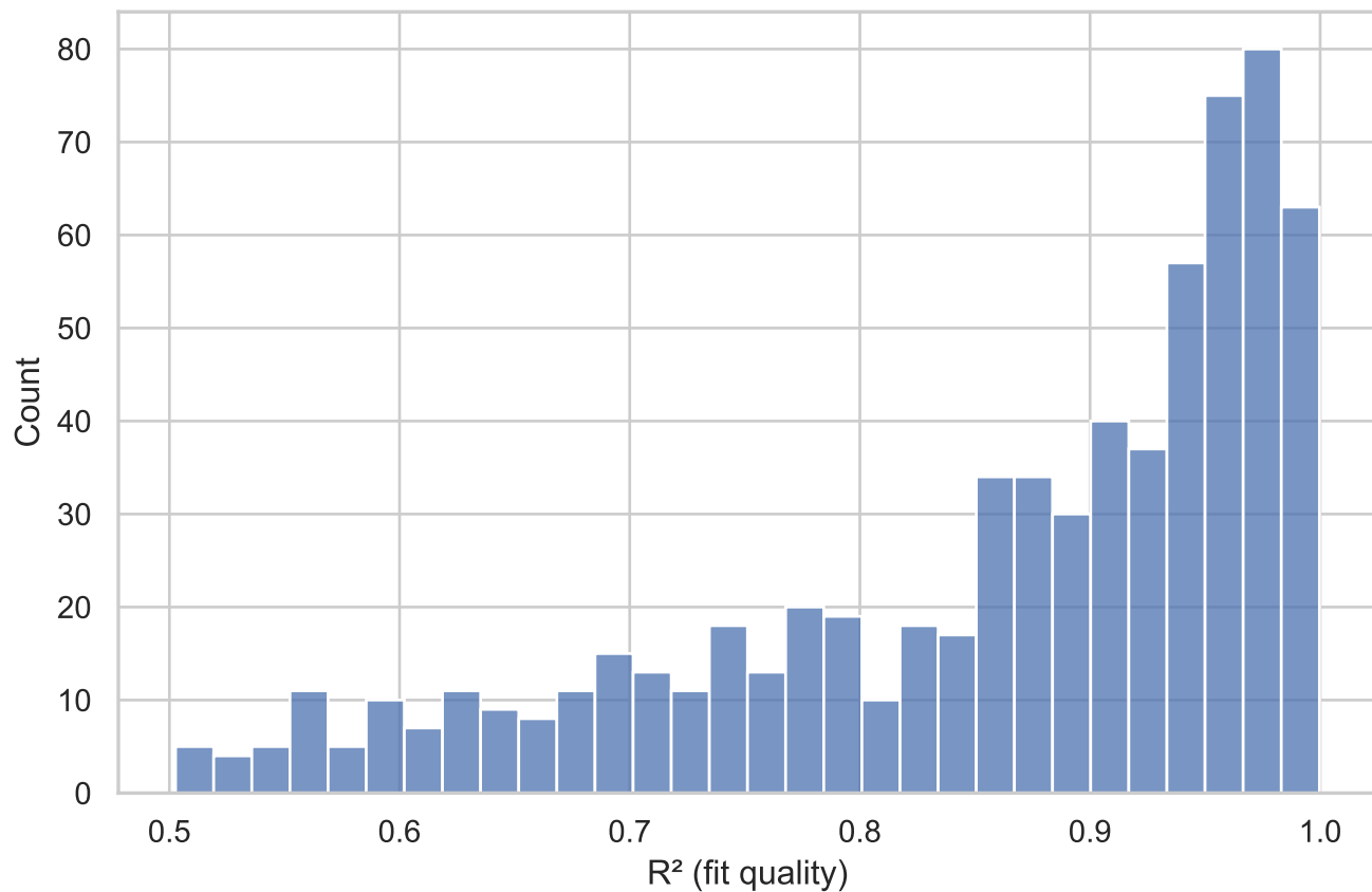
Distribution of R^2 Values
