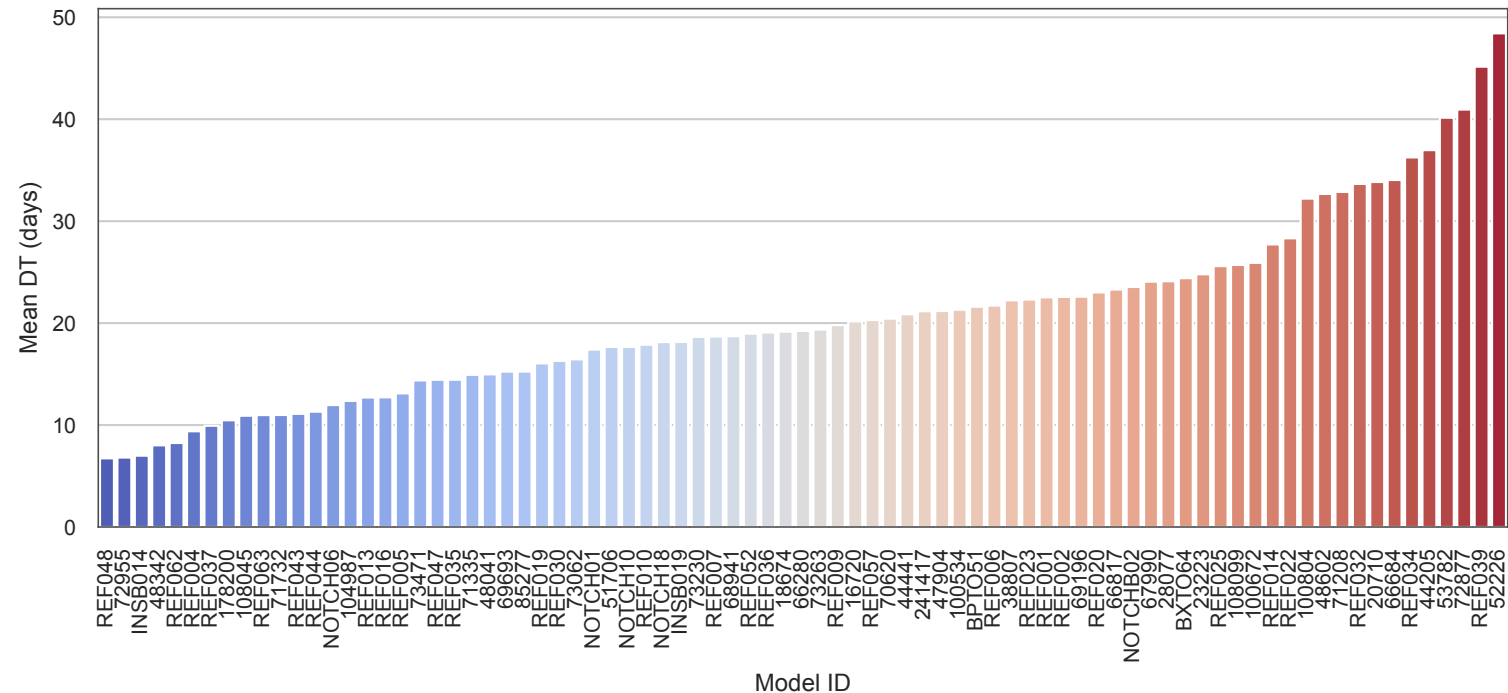
Model-wise doubling times (sorted)
