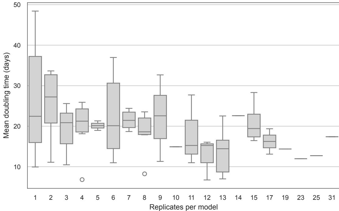
Effect of replicate count on doubling time
