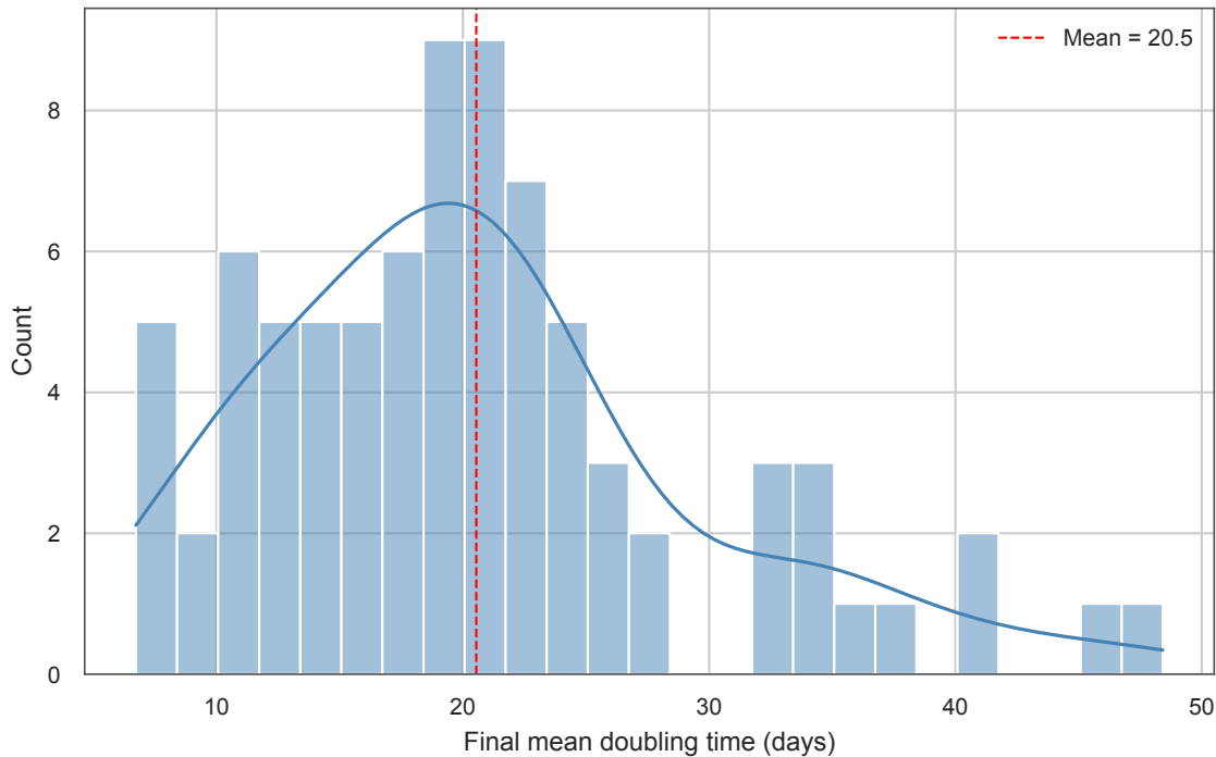
Distribution of model-level doubling times
