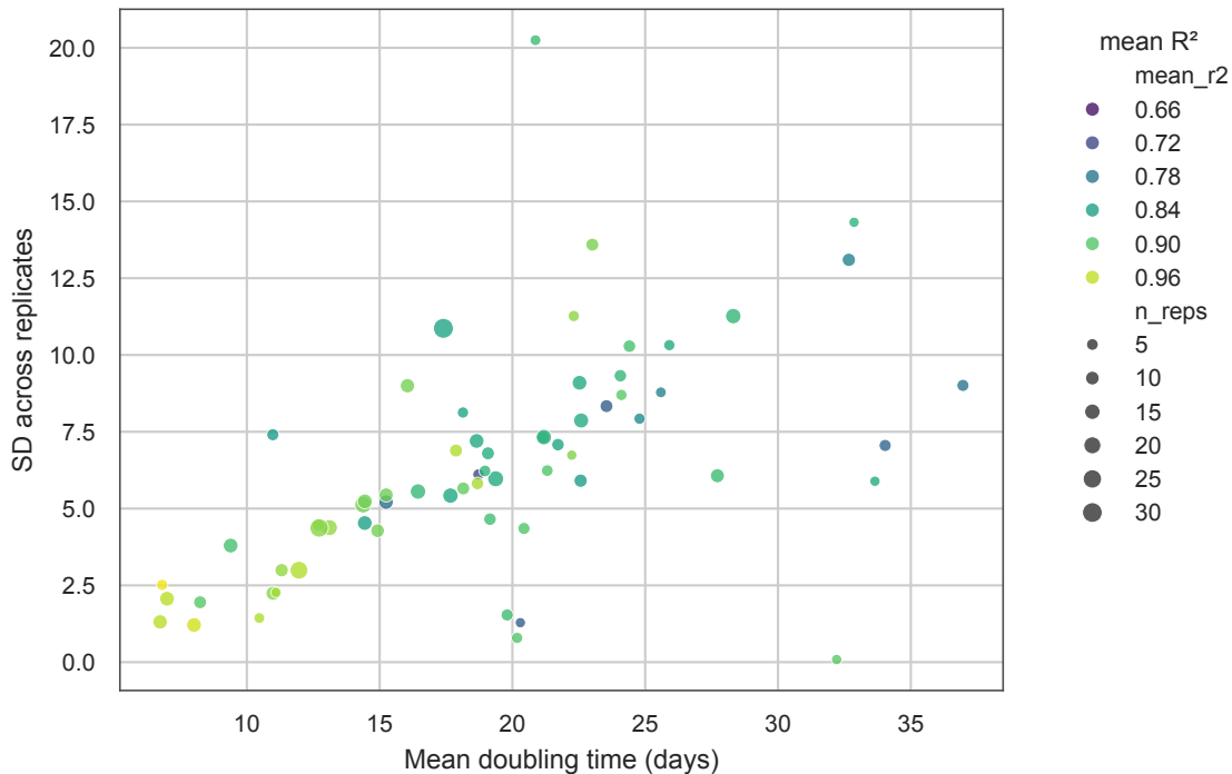
Within-model variability vs mean doubling time
