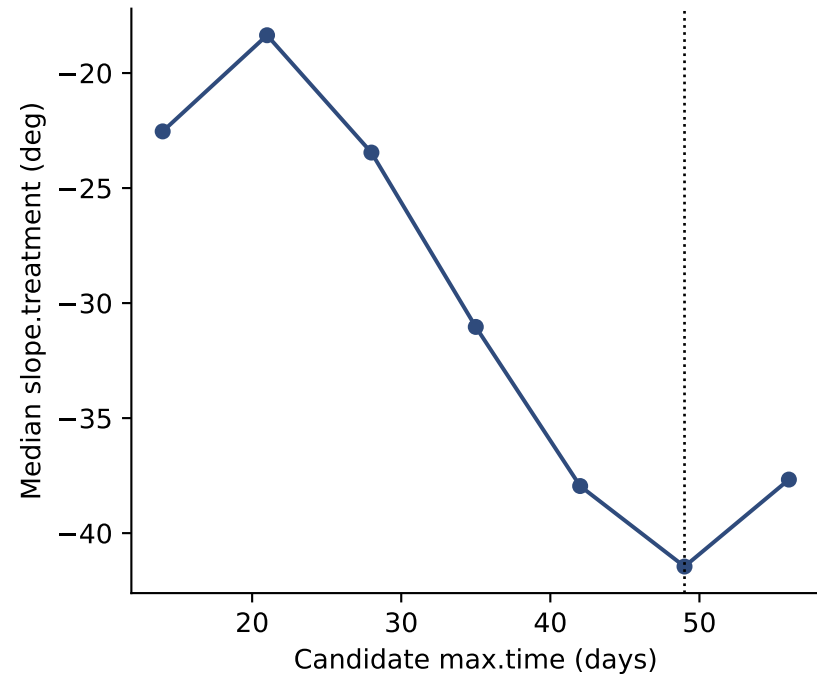
Retained-sample drift
