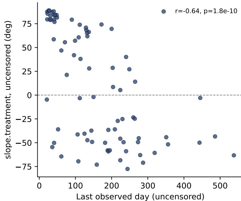
Confound check
