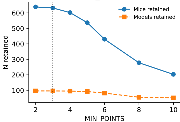
MIN_POINTS
