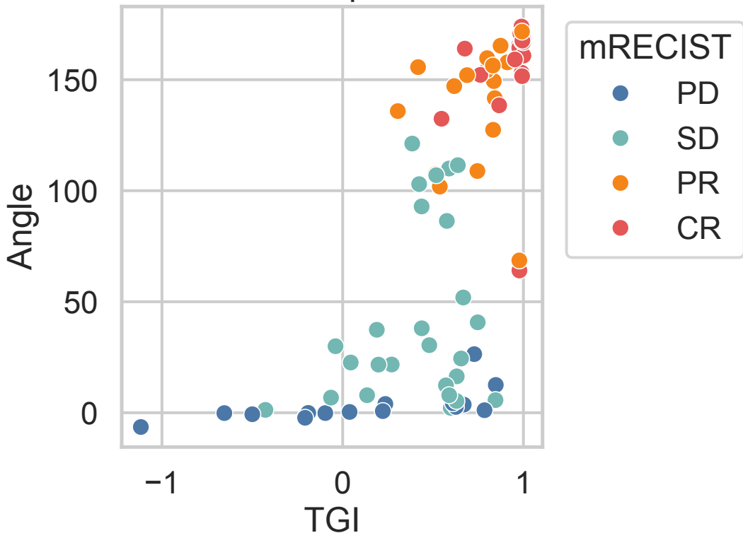
Angle vs TGI Pearson=0.64, Spearman=0.74
