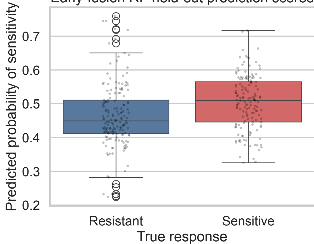
Early-fusion RF held-out prediction scores
