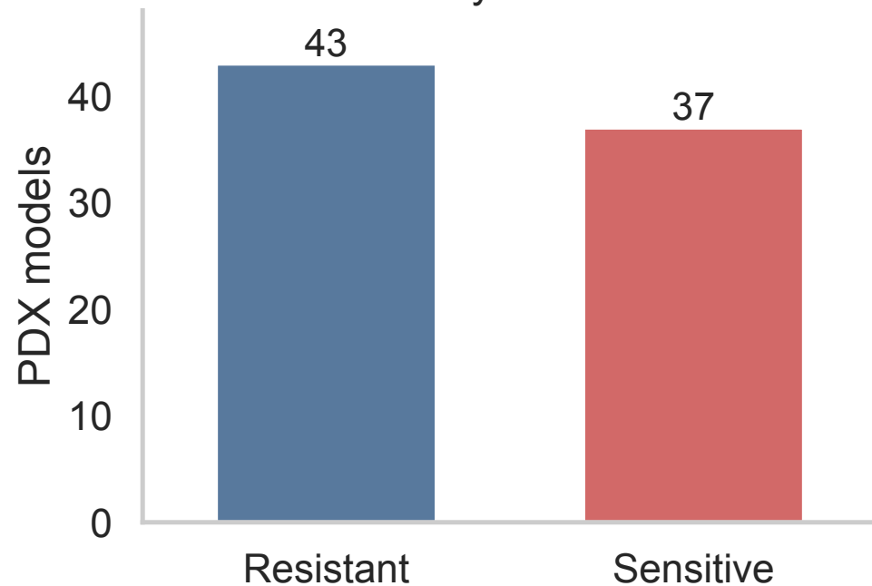
Binary classes
