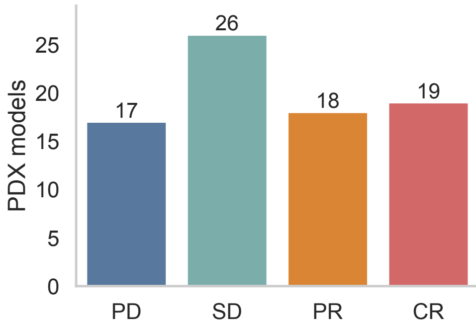
mRECIST classes
