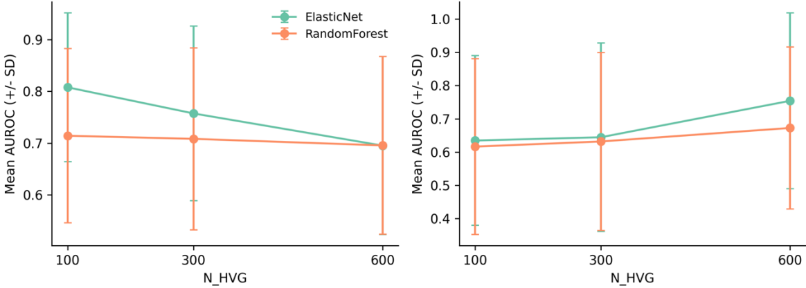
c Breast Lung
