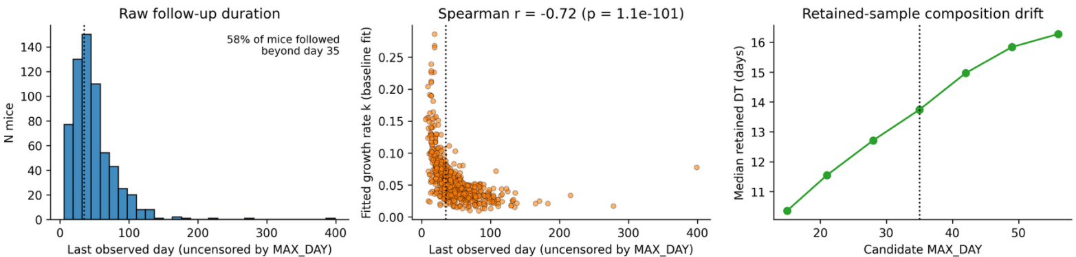
Lung: follow-up duration is confounded with growth rate
