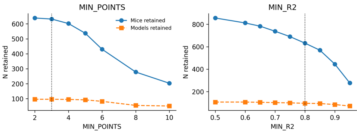
Lung: DT-fit QC threshold sensitivity
