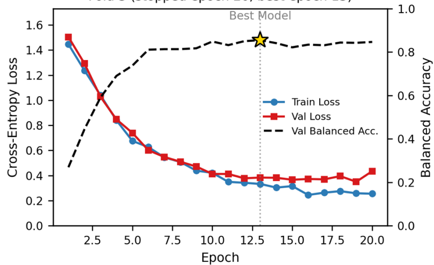
Fold 3 (stopped epoch 20, best epoch 13)
