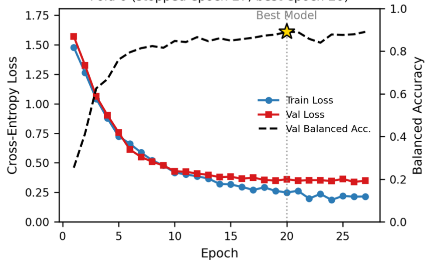
Fold 0 (stopped epoch 27, best epoch 20)
