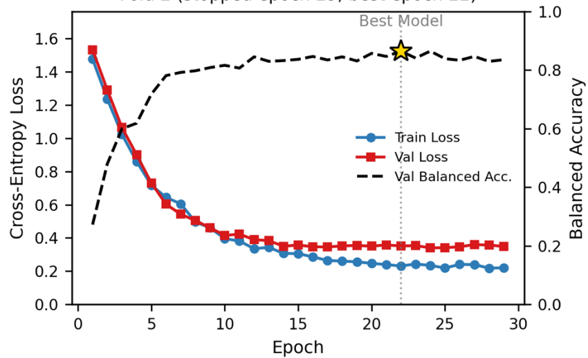
Fold 2 (stopped epoch 29, best epoch 22)
