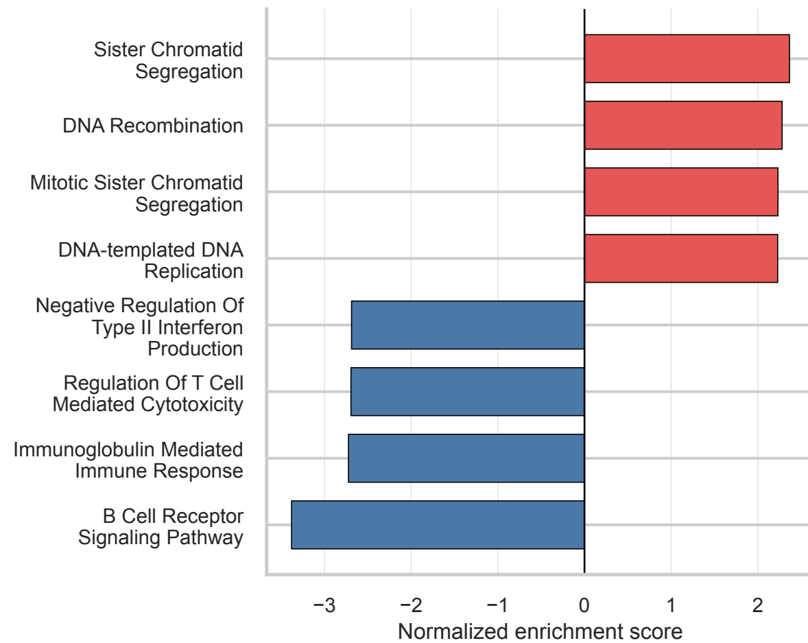
GO Biological Process
