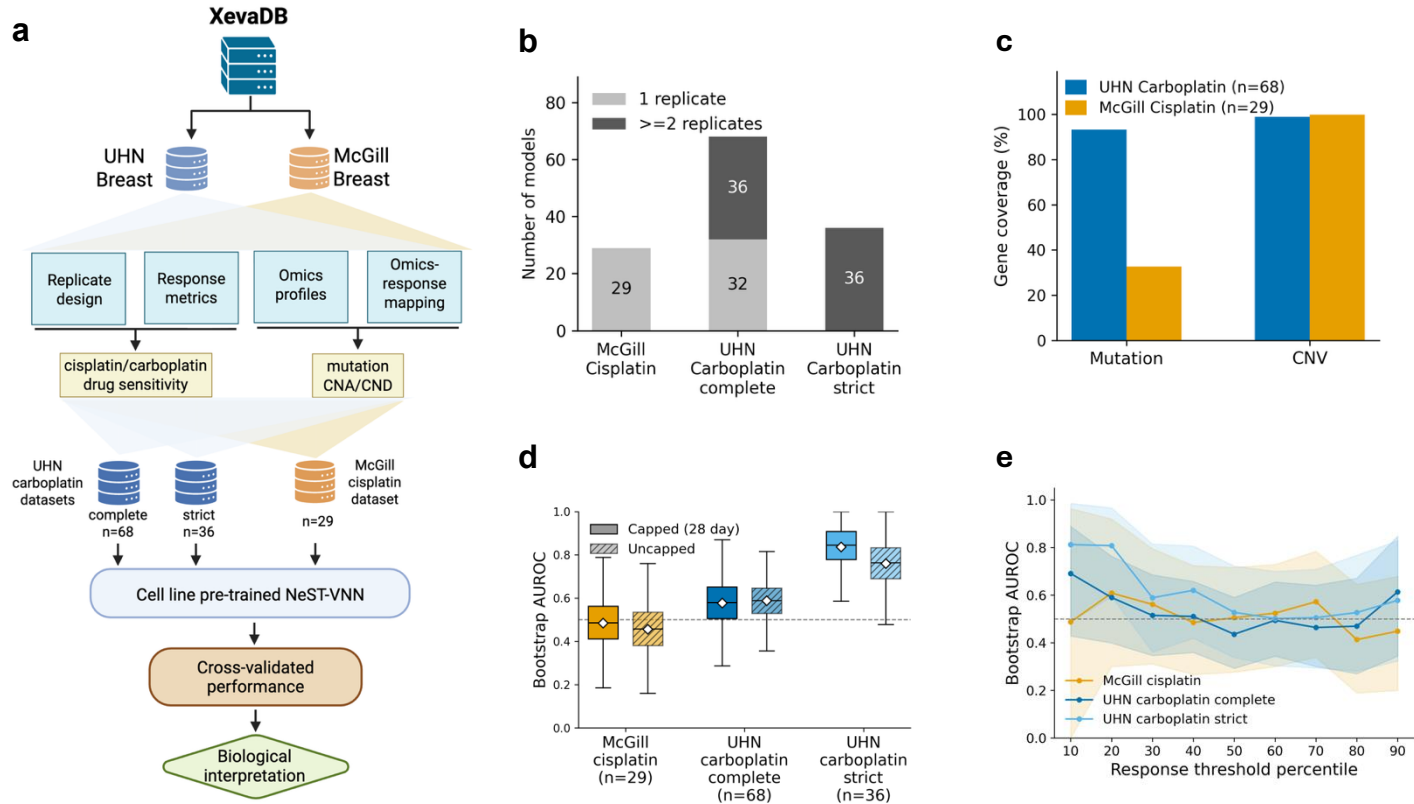
Figure 4. Cross-platform validation of NeST-VNN on independent PDX cohorts.
