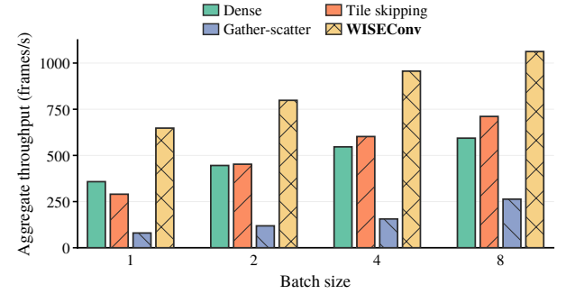
Figure 6. Stream-level batch sensitivity for YOLOv8n on RTX 3080. Eight disjoint segments of MOT16-03 provide a fixed population of temporal transitions across batch sizes, and each lane maintains independent temporal state. Dense, tile skipping, and WISEConv use CUDA Graphs; gather-scatter remains eager because its active count changes the GEMM shape. Higher is better.
