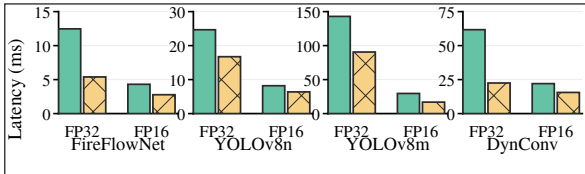
(b) AGX Orin
