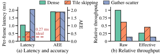
Figure 1. FireFlowNet [28] using the Ev-Conv [8] event-driven mask policy on MVSEC [45] and RTX 3080, comparing cuDNN (Dense), DeltaCNN tile skipping [30], and MMCV’s native gather-scatter path [5]. (a) Mean full-model per-frame latency and average endpoint error (AEE; lower is better). The dashed line marks dense latency scaled by the active ratio aggregated across layers; the sparse paths use the same masks and produce nearly identical AEE. (b) Raw throughput T and effective throughput T_{\text{eff}} , each normalized to dense raw throughput. The dense useful-compute ratio equals the active ratio set by the Ev-Conv mask policy ( \alpha \approx 26.3\% ).
