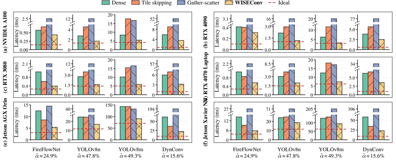
Figure 3. Full-model mean per-frame latency across GPU platforms. Each workload uses an independent y-axis. Labels report the model-level active ratio \hat{\alpha} , aggregated as described in §6.1 and averaged across evaluation sequences. Red dashed lines mark ideal proportional scaling, computed by applying each sequence’s model-level active ratio to its dense latency before aggregation.
