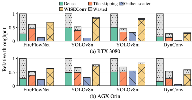
Figure 5. Full-model effective throughput \eta T and wasted throughput (1 - \eta)T on RTX 3080 and AGX Orin, normalized within each platform to Dense raw throughput.
