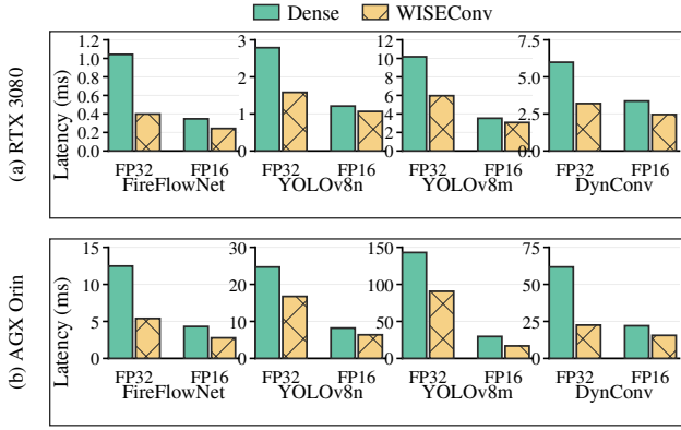
Figure 6. FP32 (SIMT) vs. FP16 (tensor core) full-model latency for Dense and WISEConv across all four workloads. FP16 WISEConv values for YOLOv8n and YOLOv8m are estimates from per-layer profiling.
