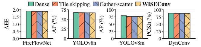
Figure 4. Task accuracy on RTX 3080 under the evaluated upstream sparsity policies, measured by AEE (↓), AP (↑), and PCKh (↑).
