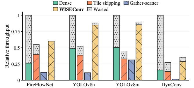
Figure 5. Full-model effective throughput \eta T and wasted throughput (1 - \eta)T on RTX 3080, normalized to dense raw throughput.
