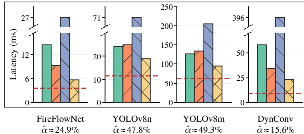
(f) Jetson Xavier NX
