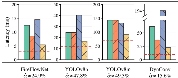
(e) Jetson AGX Orin
