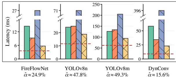
(f) Jetson Xavier NX
