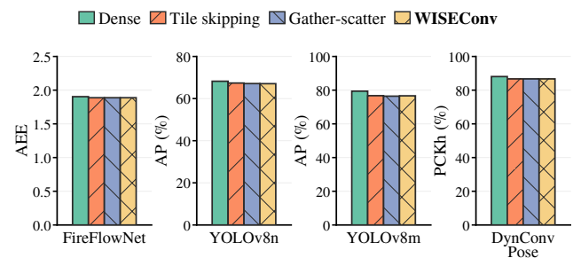
Figure 4. Task accuracy at the operating points used in the end-to-end experiments. AEE is lower-is-better; AP and PCKh are higher-is-better. We report accuracy once on RTX 3080 because the models, inputs, and upstream masks are shared across platforms.
