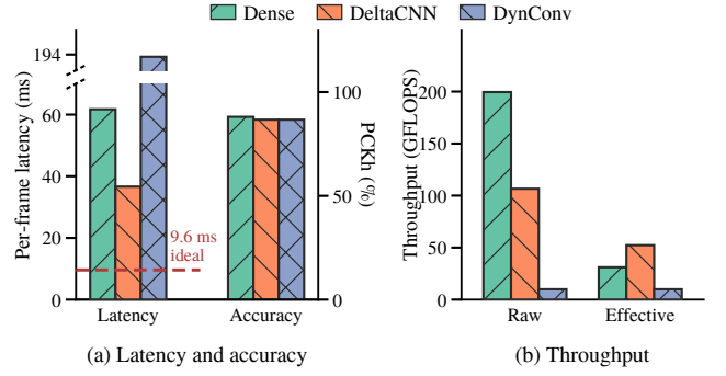
Fig. 1. Statistics of DynConv [5], a pose estimator with learned spatial gating, on the MPII human-pose dataset [13] and Jetson AGX Orin, comparing the native cuDNN path (Dense) against the two sparse paths. (a) End-to-end average per-frame latency (left axis; the dashed line marks the dense latency scaled by the active ratio aggregated across layers) and PCKh accuracy (right axis; PCKh evaluates the percentage of keypoints localized within half the head size). The sparse paths apply the same mask, so their accuracy coincides. (b) Raw throughput T and effective throughput T_{eff} , aggregated across the model’s convolution layers. The dense useful-compute ratio implies the active ratio set by DynConv’s spatial gating ( \alpha \approx 15.6\% ).
