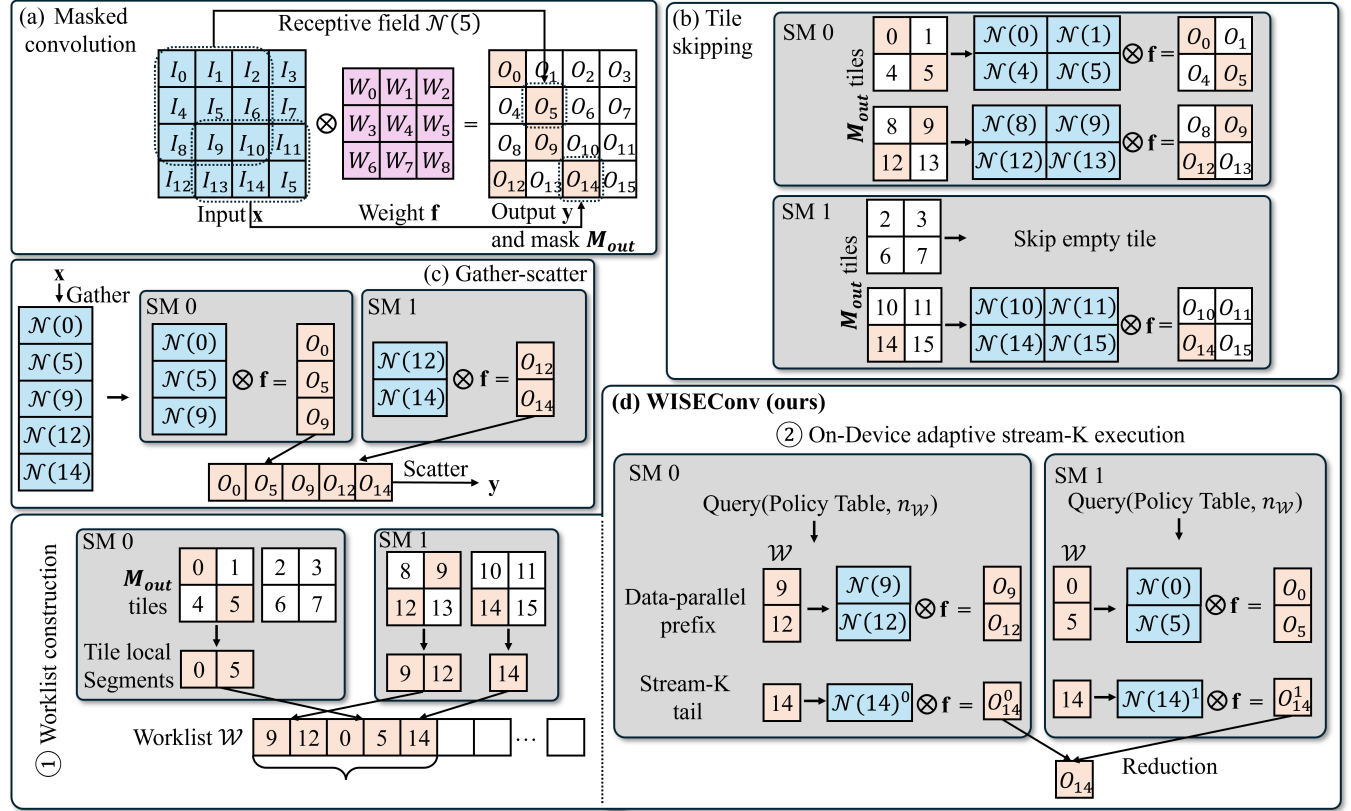
Figure 2. Overview of WISEConv and baseline execution paths. (a) Masked convolution: M_{out} marks active output positions (colored); the operator computes only these from \mathbf{x} and \mathbf{f} . (b) Tile skipping skips only fully inactive tiles; partially active tiles compute all positions. (c) Gather-scatter packs exactly the receptive fields of active positions, computes, and scatters results back. (d) WISEConv: ① constructs a tile-local worklist and ② consumes it via on-device adaptive Stream-K execution.
