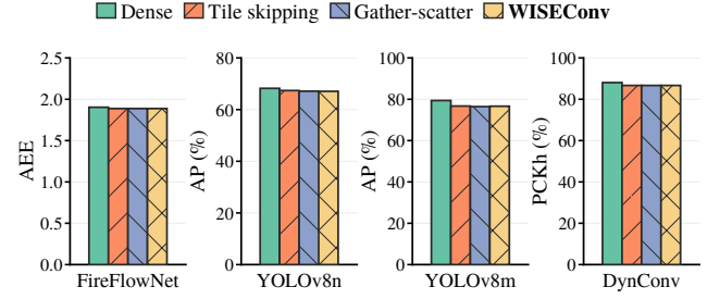
Figure 4. Task accuracy on RTX 3080 under the evaluated upstream sparsity policies, measured by AEE (↓), AP (↑), and PCKh (↑).
