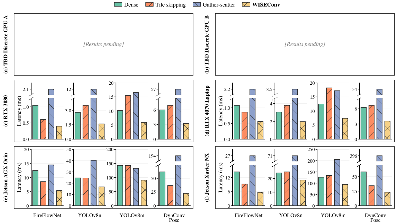
Figure 3. Full-model mean per-frame latency across GPU platforms. Within each platform, every workload uses its own y-axis to compare the four execution paths; lower is better. Broken y-axes preserve resolution where gather-scatter is substantially slower than the other paths.
