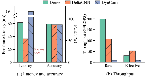
Figure 1. Statistics of DynConv [35], a pose estimator with learned spatial gating, on the MPII human-pose dataset [1] and Jetson AGX Orin, comparing the native cuDNN path (Dense) against the two sparse paths. (a) End-to-end average per-frame latency (left axis; the dashed line marks the dense latency scaled by the active ratio aggregated across layers) and PCKh accuracy (right axis; PCKh evaluates the percentage of keypoints localized within half the head size). The sparse paths apply the same mask, so their accuracy coincides. (b) Raw throughput T and effective throughput T_{\text{eff}} , aggregated across the model’s convolution layers. The dense useful-compute ratio equals the active ratio set by DynConv’s spatial gating ( \alpha \approx 15.6\% ).
