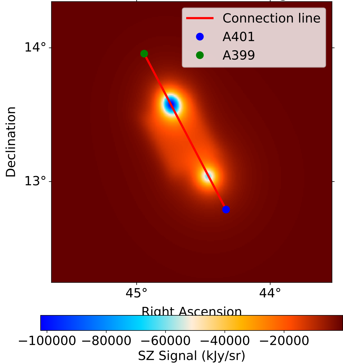
SZ Model at 98 GHz with Line Connecting A401 and A399
