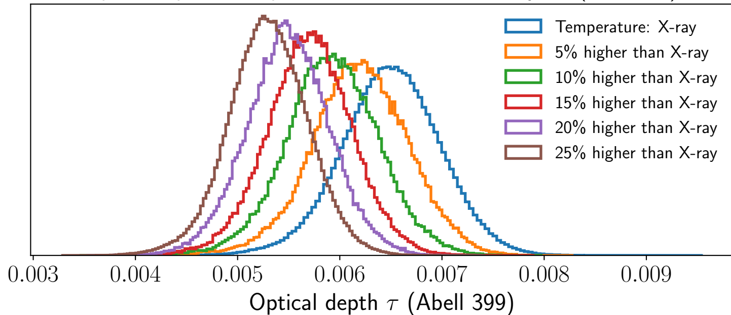
Optical depth vs temperature for individual velocity fits (Abell 399)
