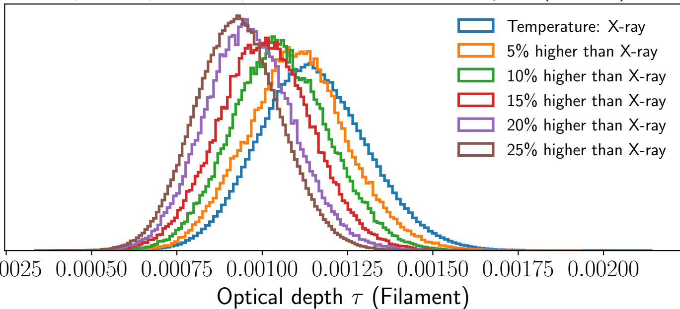
Optical depth vs temperature for individual velocity fits (filament)
