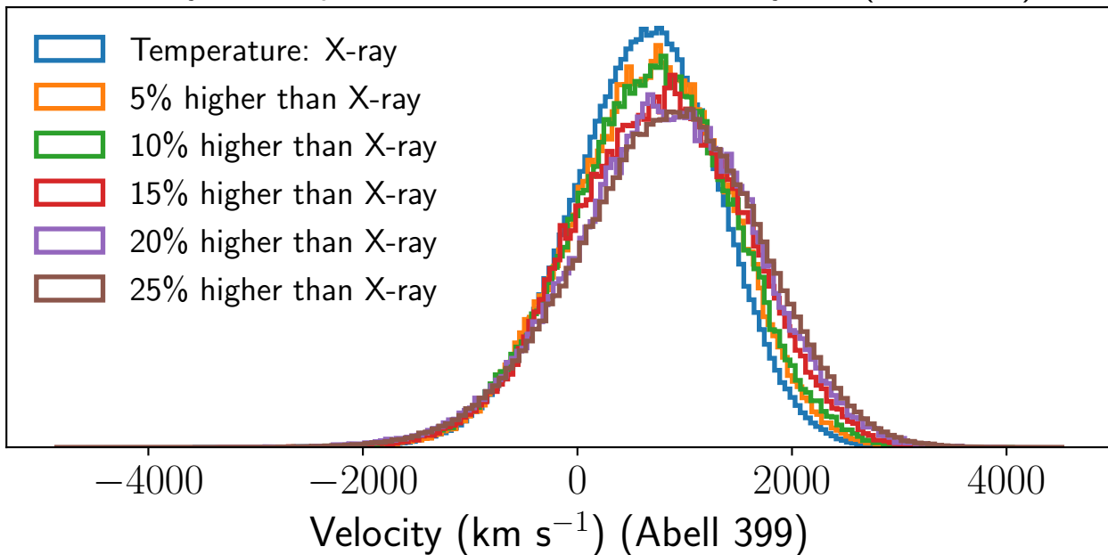
Velocity vs temperature for individual velocity fits (Abell 399)
