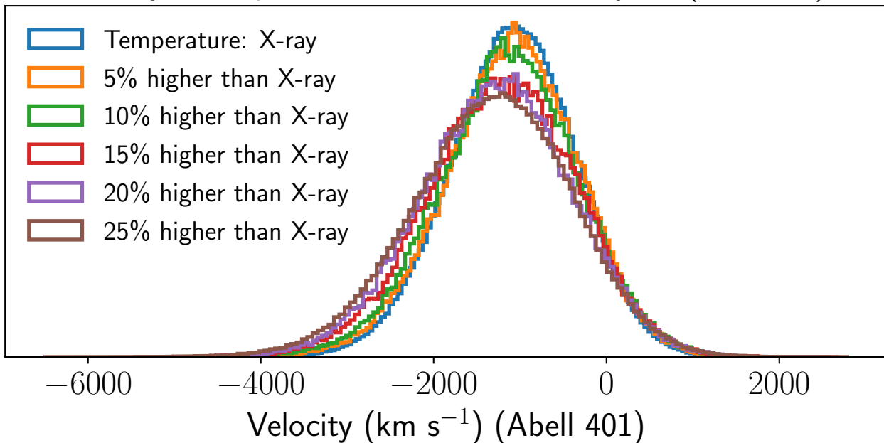
Velocity vs temperature for individual velocity fits (Abell 401)
