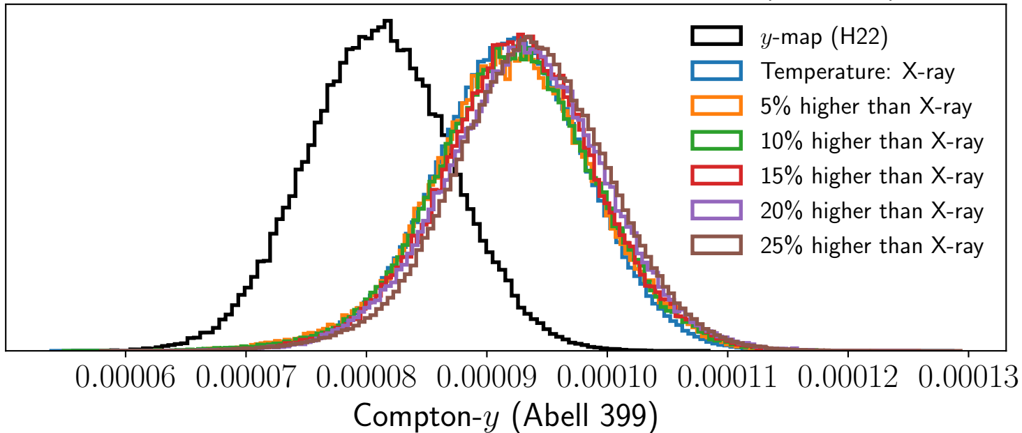
Compton- y vs temperature for individual velocity fits (Abell 399)
