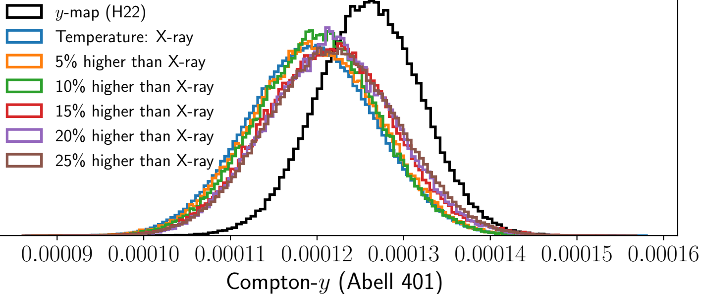
Compton- y vs temperature for individual velocity fits (Abell 401)
