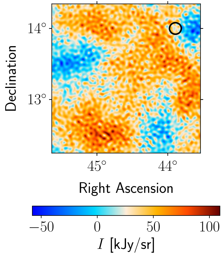
Residual: Planck 100 GHz
