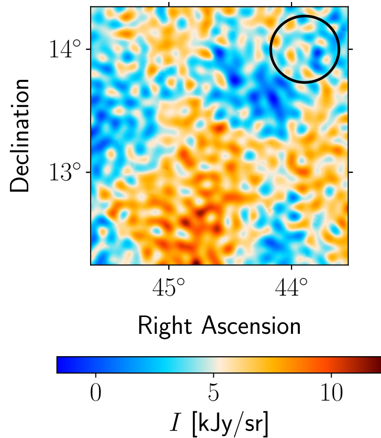
Residual: Planck 30 GHz
